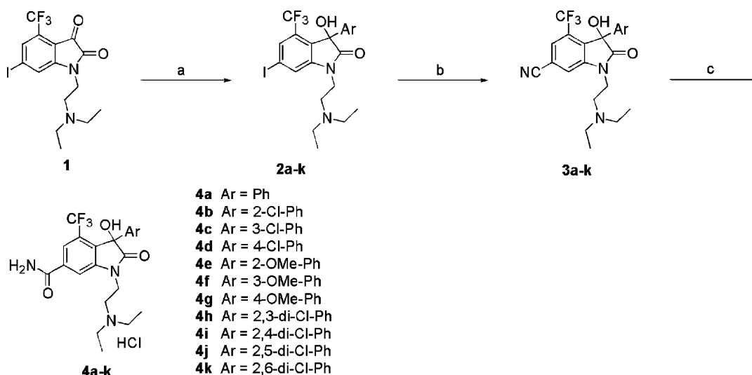
Scheme 1. Reagents and conditions: (a) ArMgBr, THF, 0 °C or ArLi, THF, –78 °C, 32–71%; (b) Zn(CN) 2 , Pd(PPh 3 ) 4 , DMF, 80 °C, 48–95%; (c) (1) powdered KOH, tert -butyl alcohol, 50 °C, (2) HCl, dioxane, rt, 61–100% (two steps).
