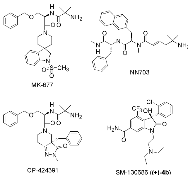
Figure 1. Structures of small molecule growth hormone secretagogues.
